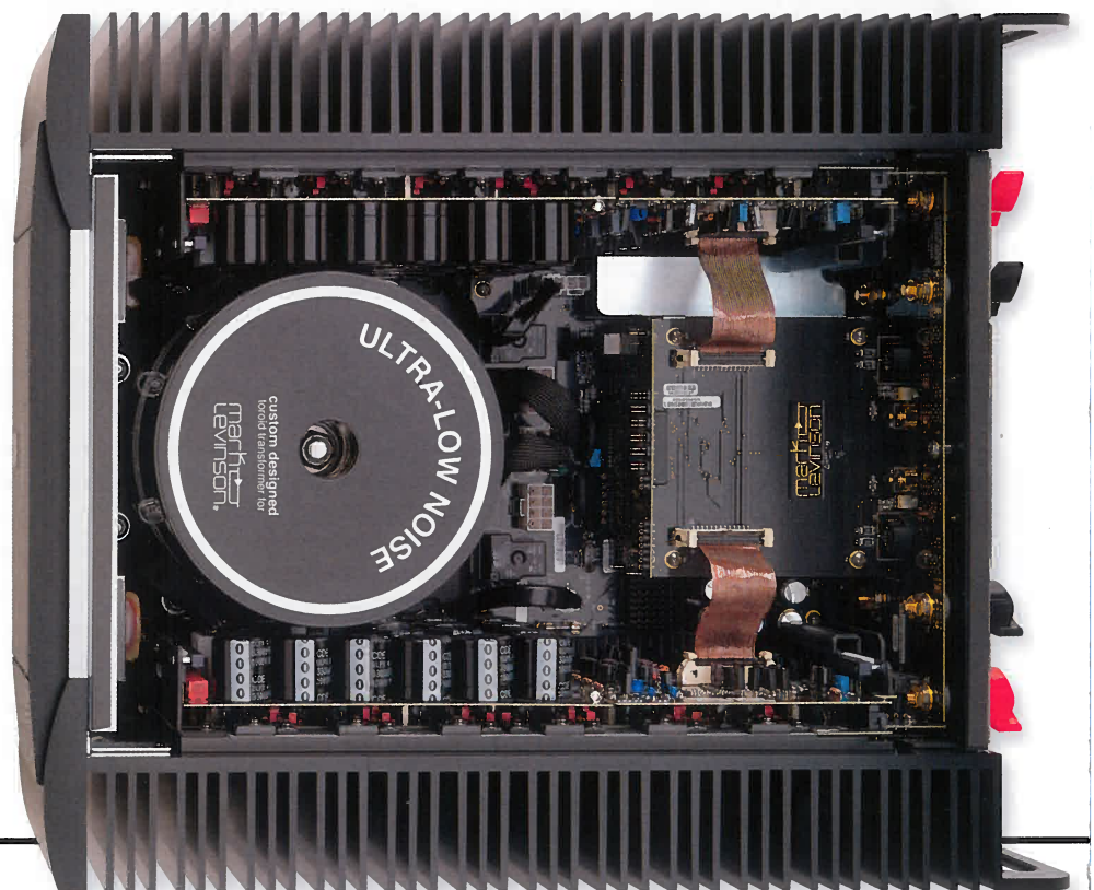
RIGHT: Massive 1800VA toroidal transformer is at the heart of a PSU that drives two fully symmetrical (balanced) Class AB amp modules, each hosting 12 high-current transistors. Temp reaches a warm 45°C across the finned heatsink
